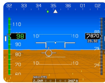
Basic PFD
